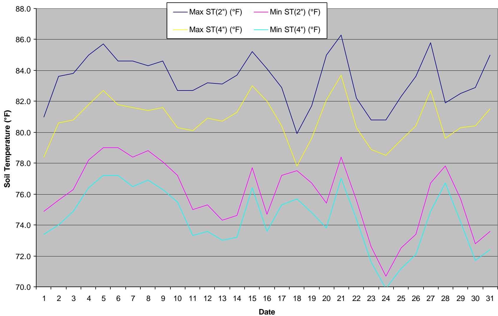
Prairie Fork Conservation Area Soil Temperature Chart (July 2003)
