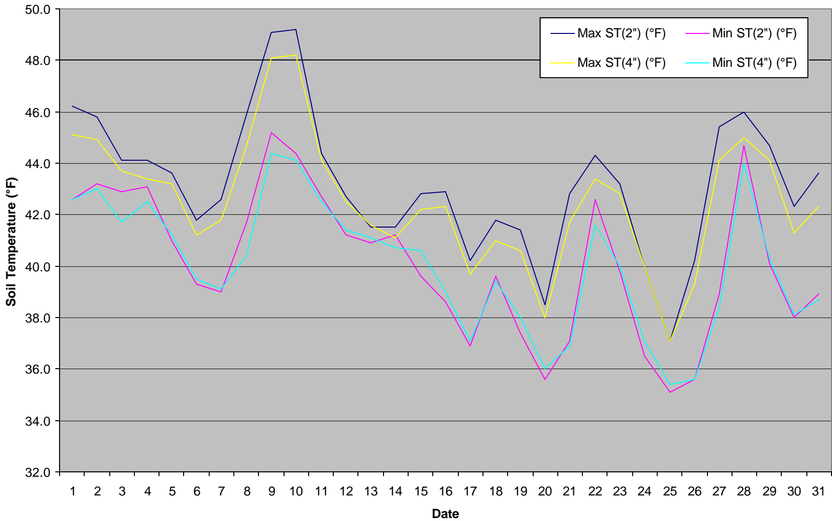
Prairie Fork Conservation Area Soil Temperature Chart (December 2003)
